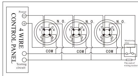
4 wire detectors wiring diagram
