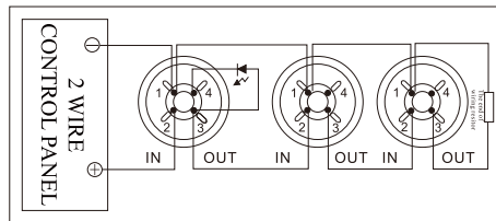
2 wire detectors wiring diagram
